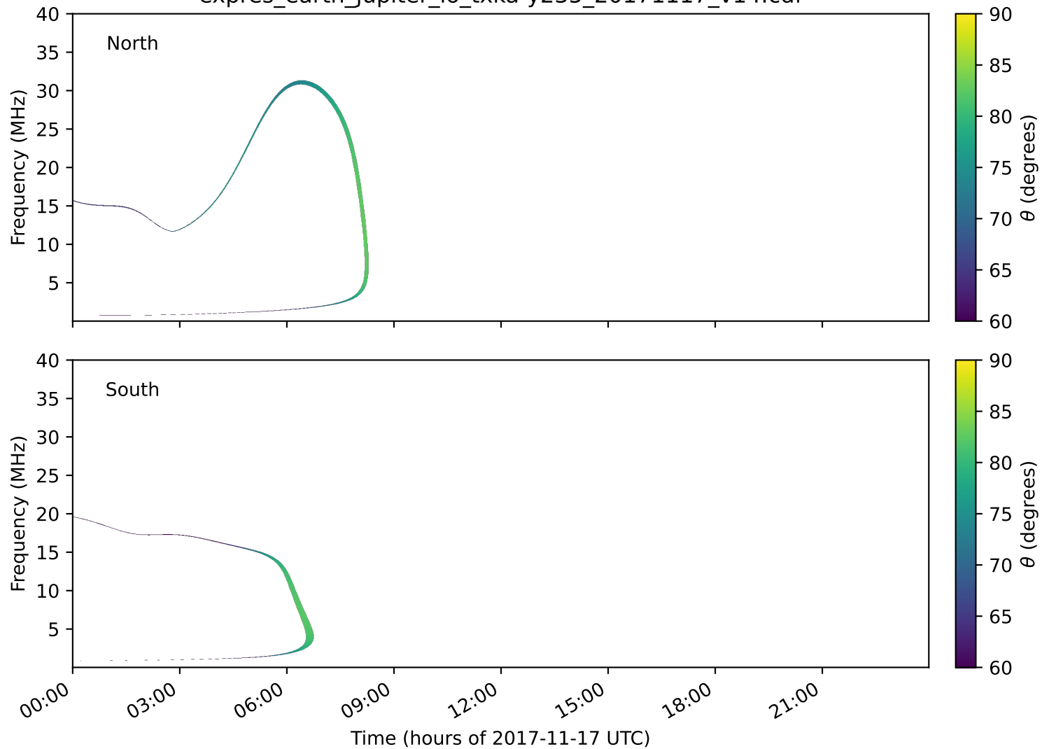
expres_earth_jupiter_io_txka-y235_20171117_v14.cdf
