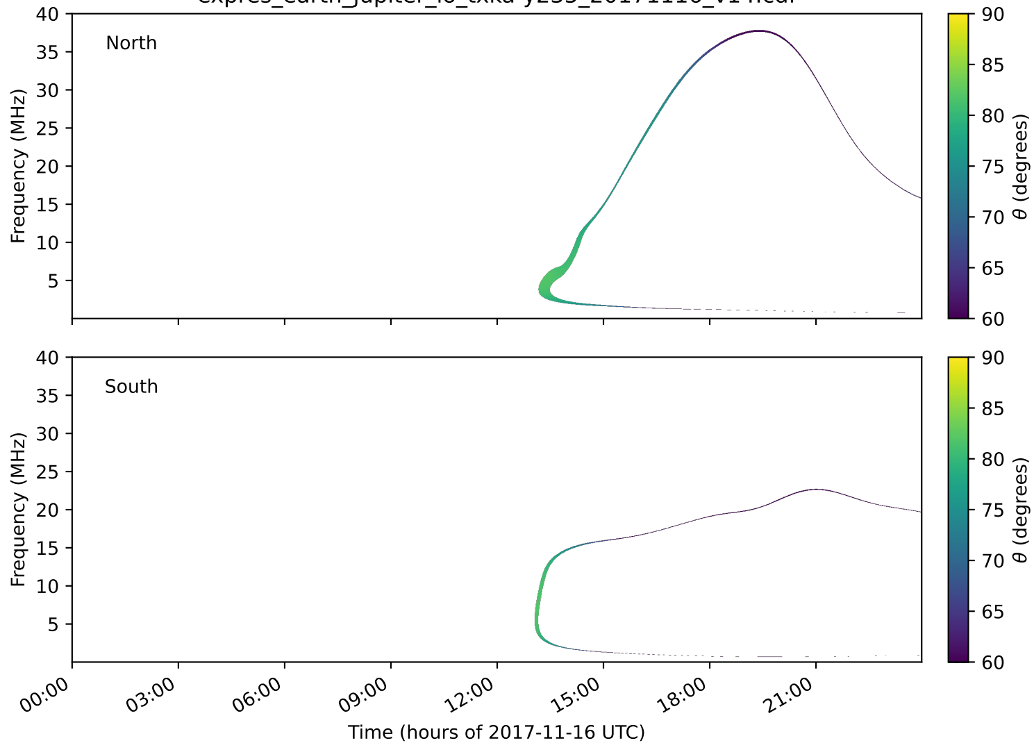
expres_earth_jupiter_io_txka-y235_20171116_v14.cdf
