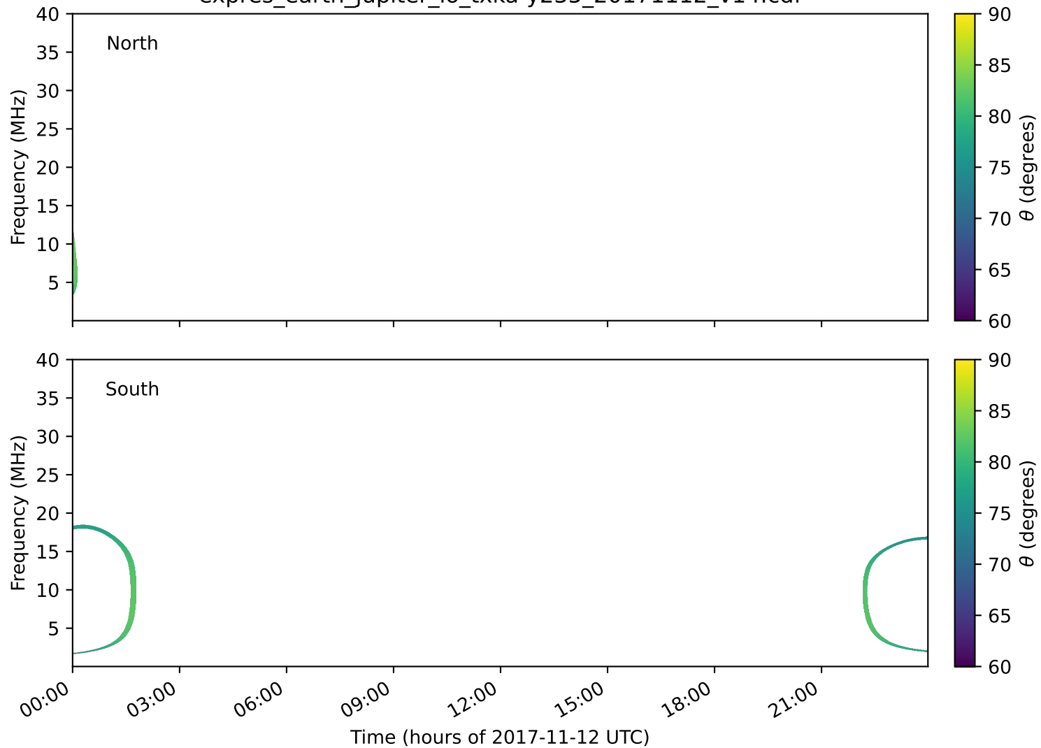
expres_earth_jupiter_io_txka-y235_20171112_v14.cdf
