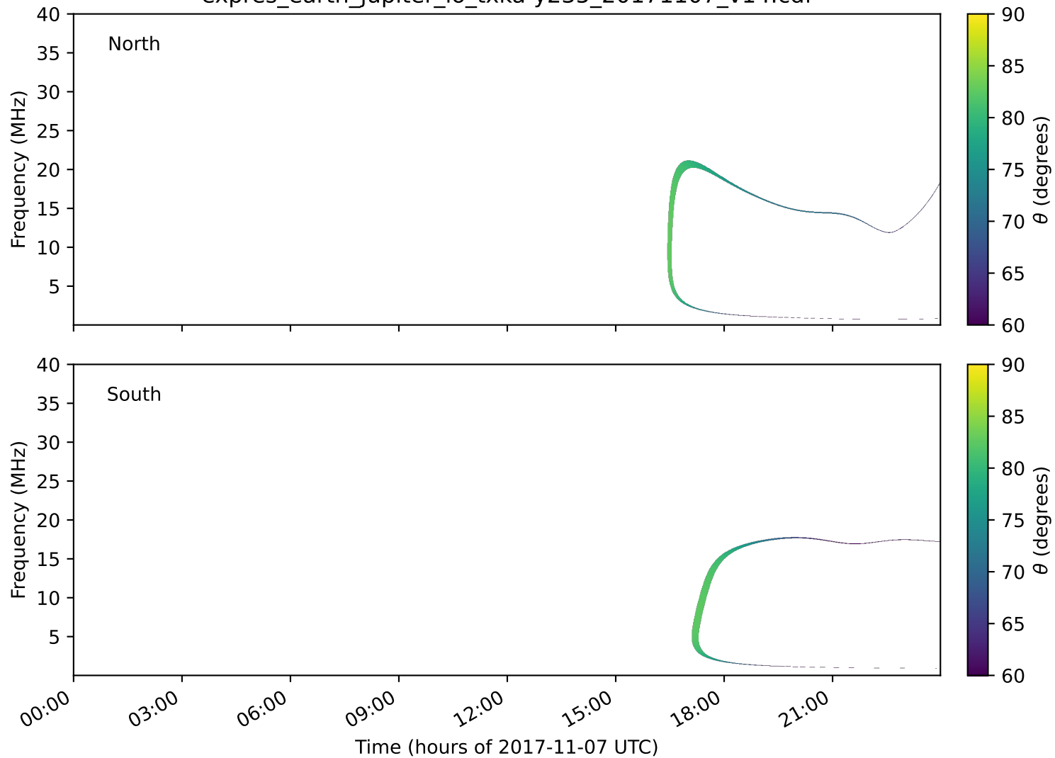
expres_earth_jupiter_io_txka-y235_20171107_v14.cdf
