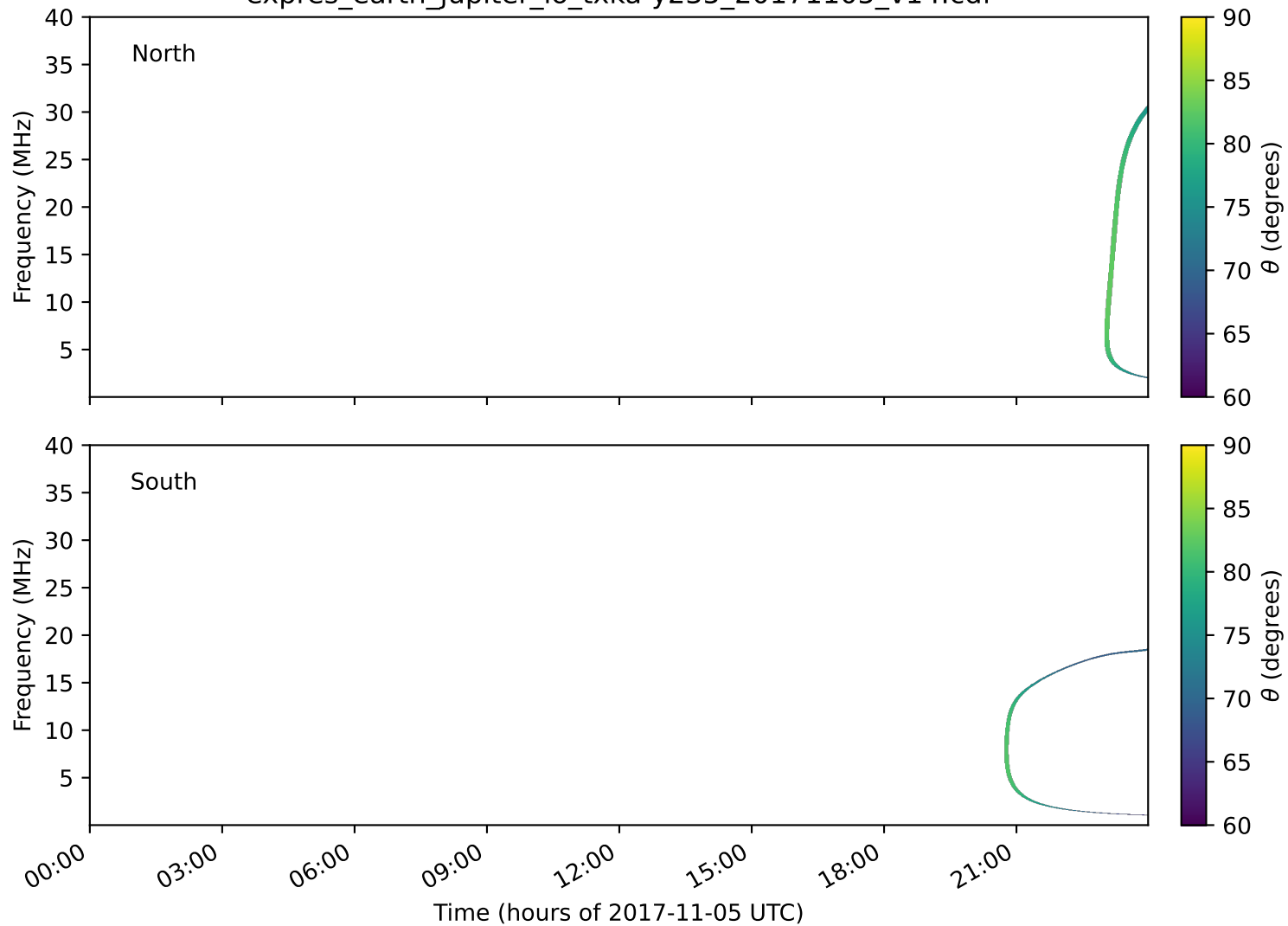
expres_earth_jupiter_io_txka-y235_20171105_v14.cdf
