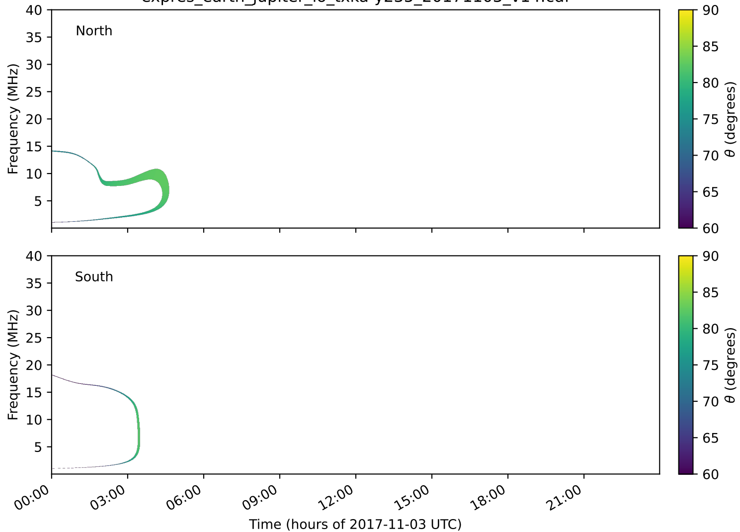
expres_earth_jupiter_io_txka-y235_20171103_v14.cdf
