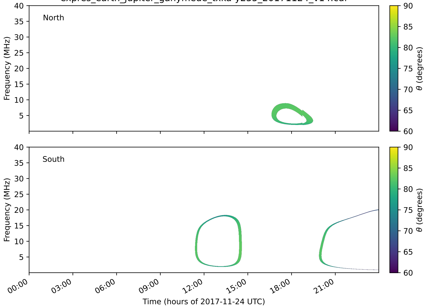
expres_earth_jupiter_ganymede_txka-y235_20171124_v14.cdf
