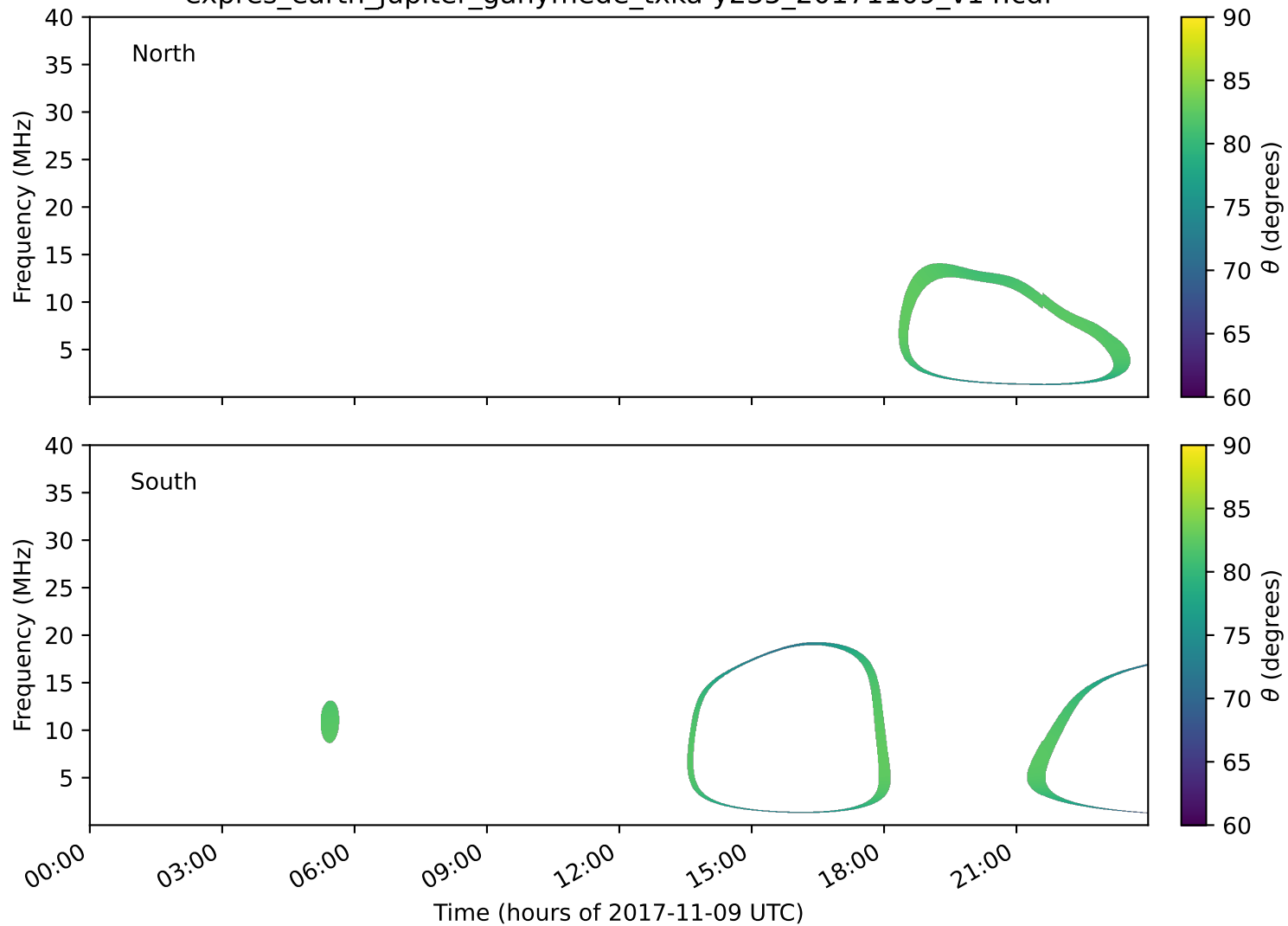
expres_earth_jupiter_ganymede_txka-y235_20171109_v14.cdf
