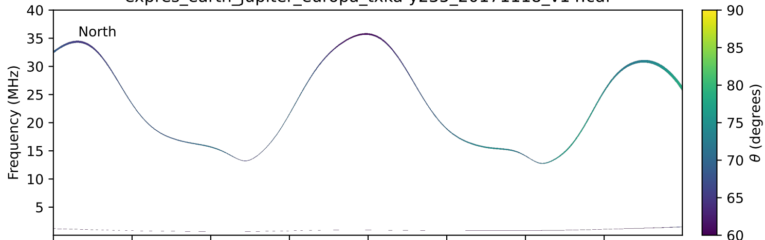
expres_earth_jupiter_europa_txka-y235_20171118_v14.cdf
