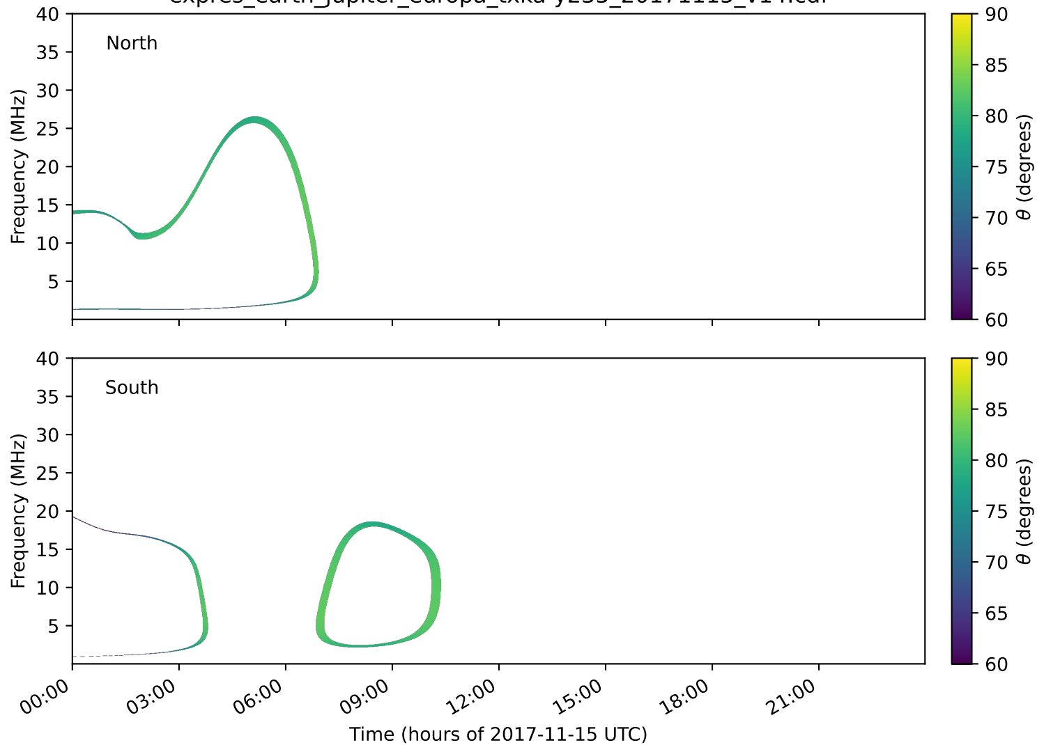
expres_earth_jupiter_europa_txka-y235_20171115_v14.cdf
