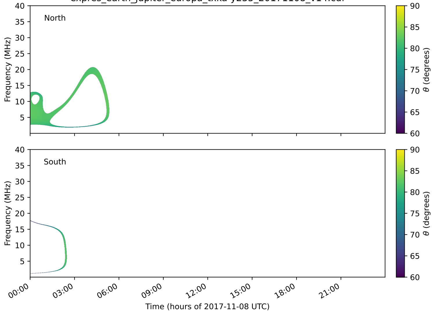
expres_earth_jupiter_europa_txka-y235_20171108_v14.cdf
