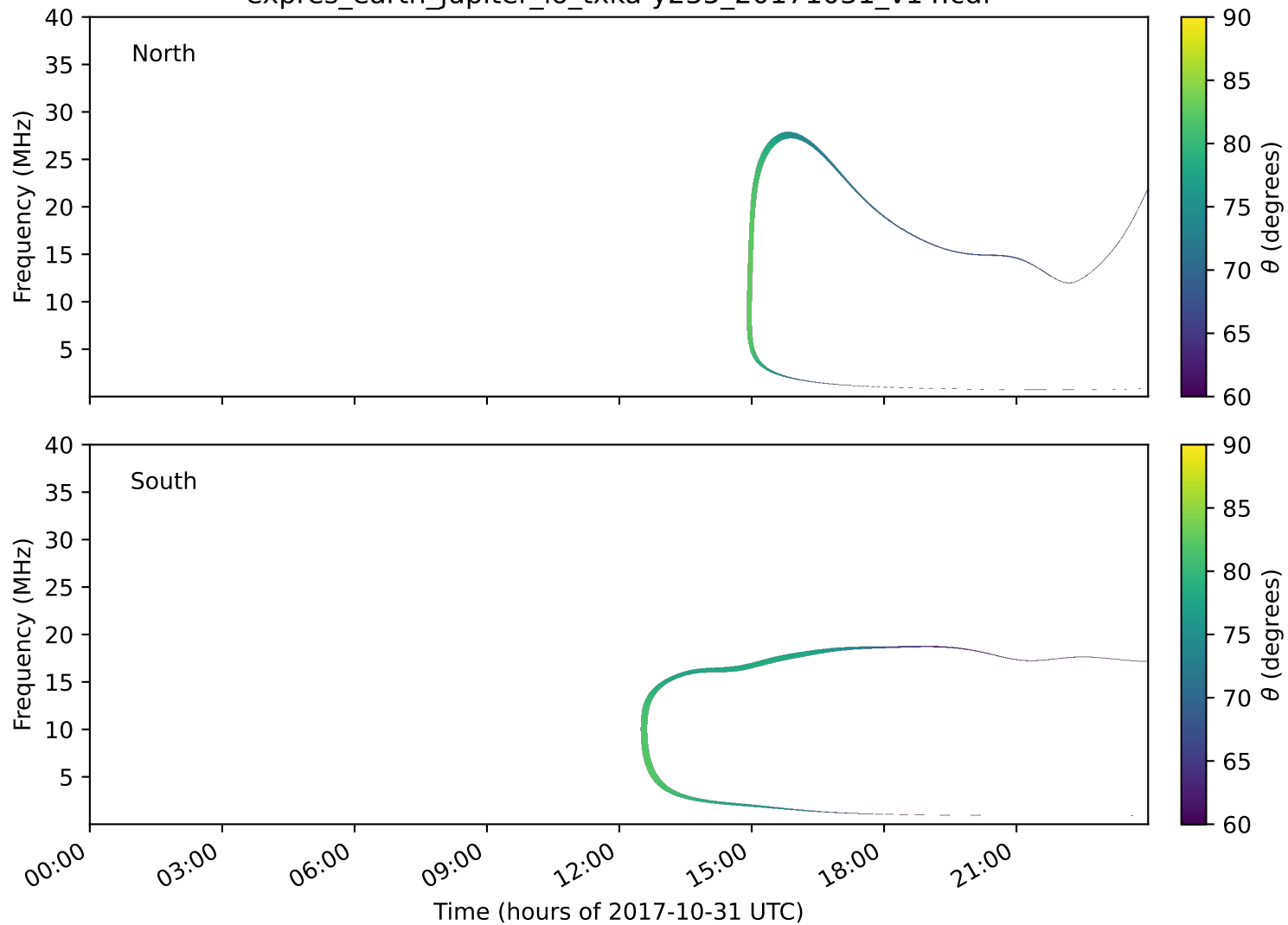
expres_earth_jupiter_io_txka-y235_20171031_v14.cdf
