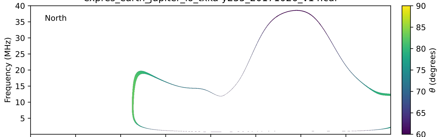
expres_earth_jupiter_io_txka-y235_20171026_v14.cdf
