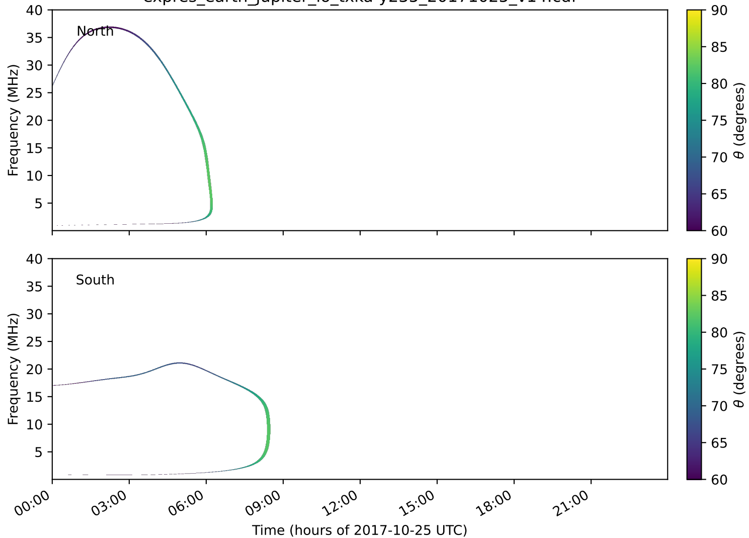
expres_earth_jupiter_io_txka-y235_20171025_v14.cdf
