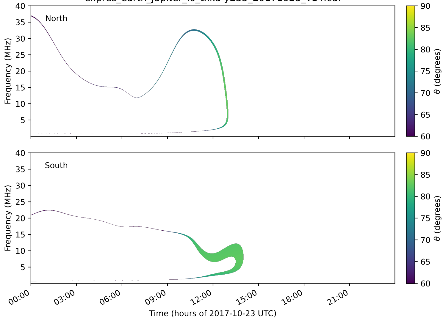
expres_earth_jupiter_io_txka-y235_20171023_v14.cdf
