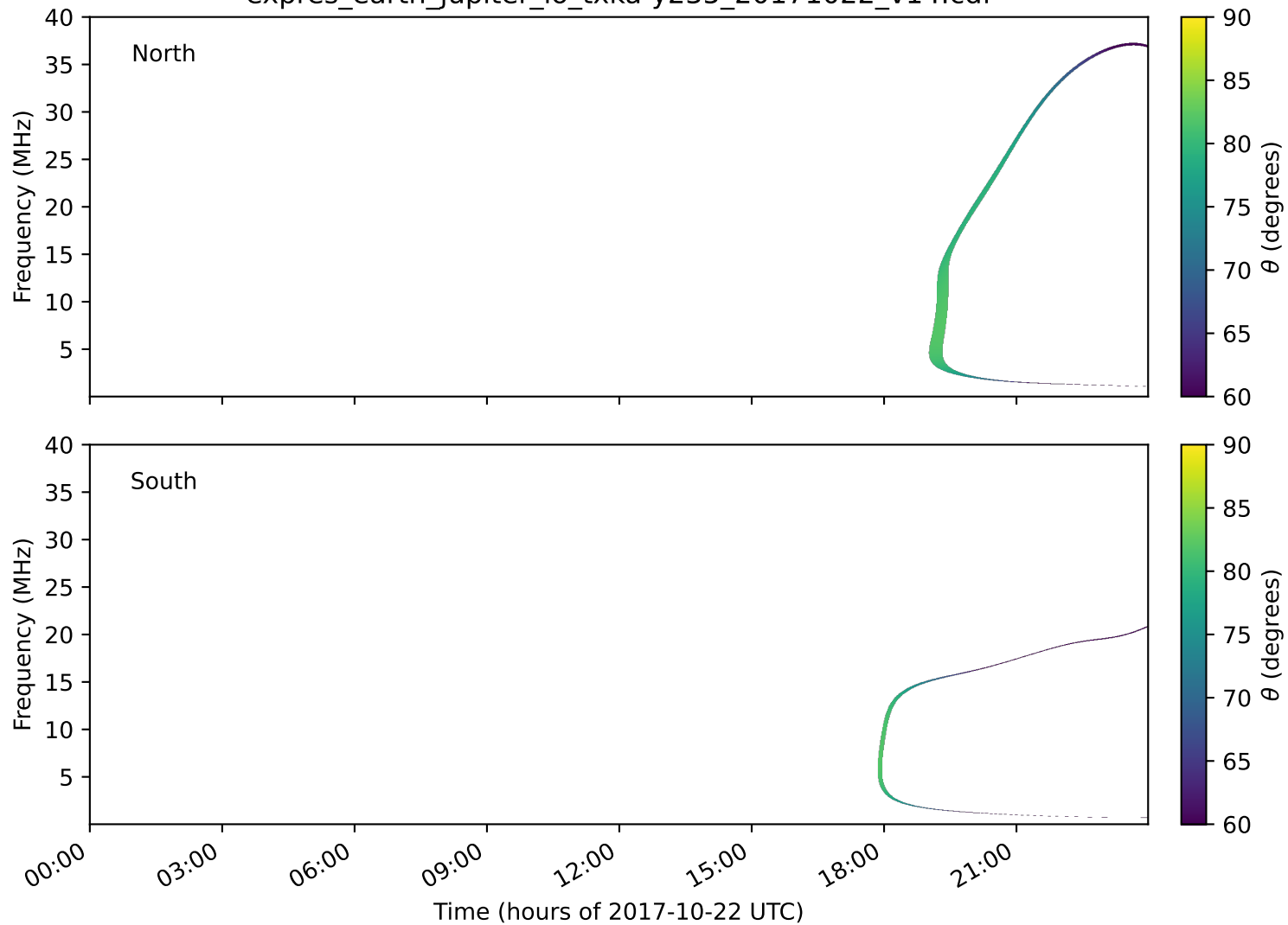
expres_earth_jupiter_io_txka-y235_20171022_v14.cdf
