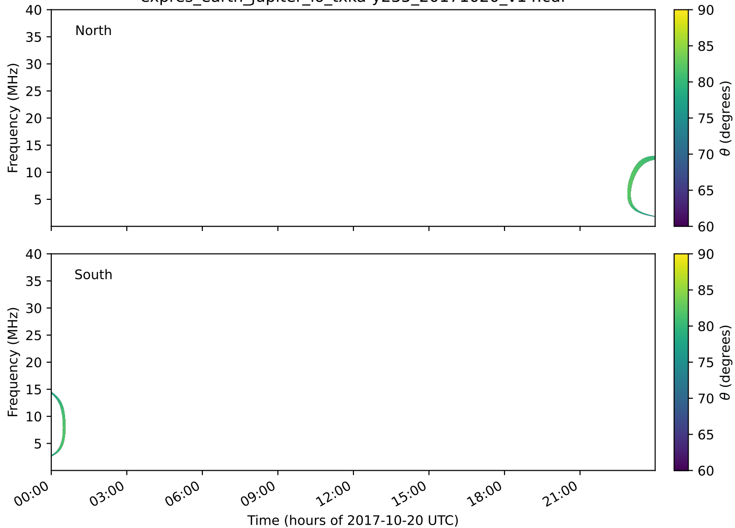
expres_earth_jupiter_io_txka-y235_20171020_v14.cdf
