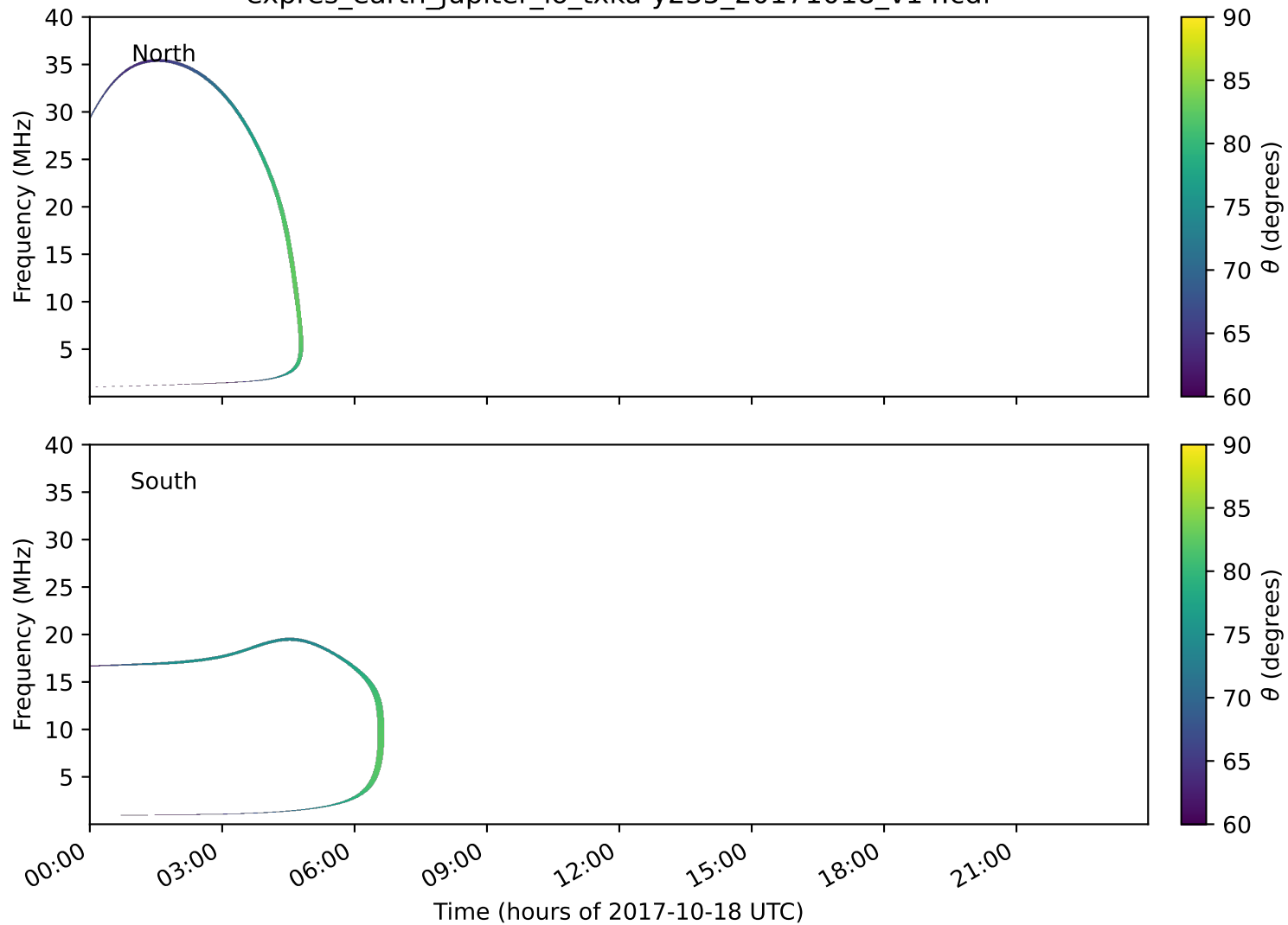
expres_earth_jupiter_io_txka-y235_20171018_v14.cdf
