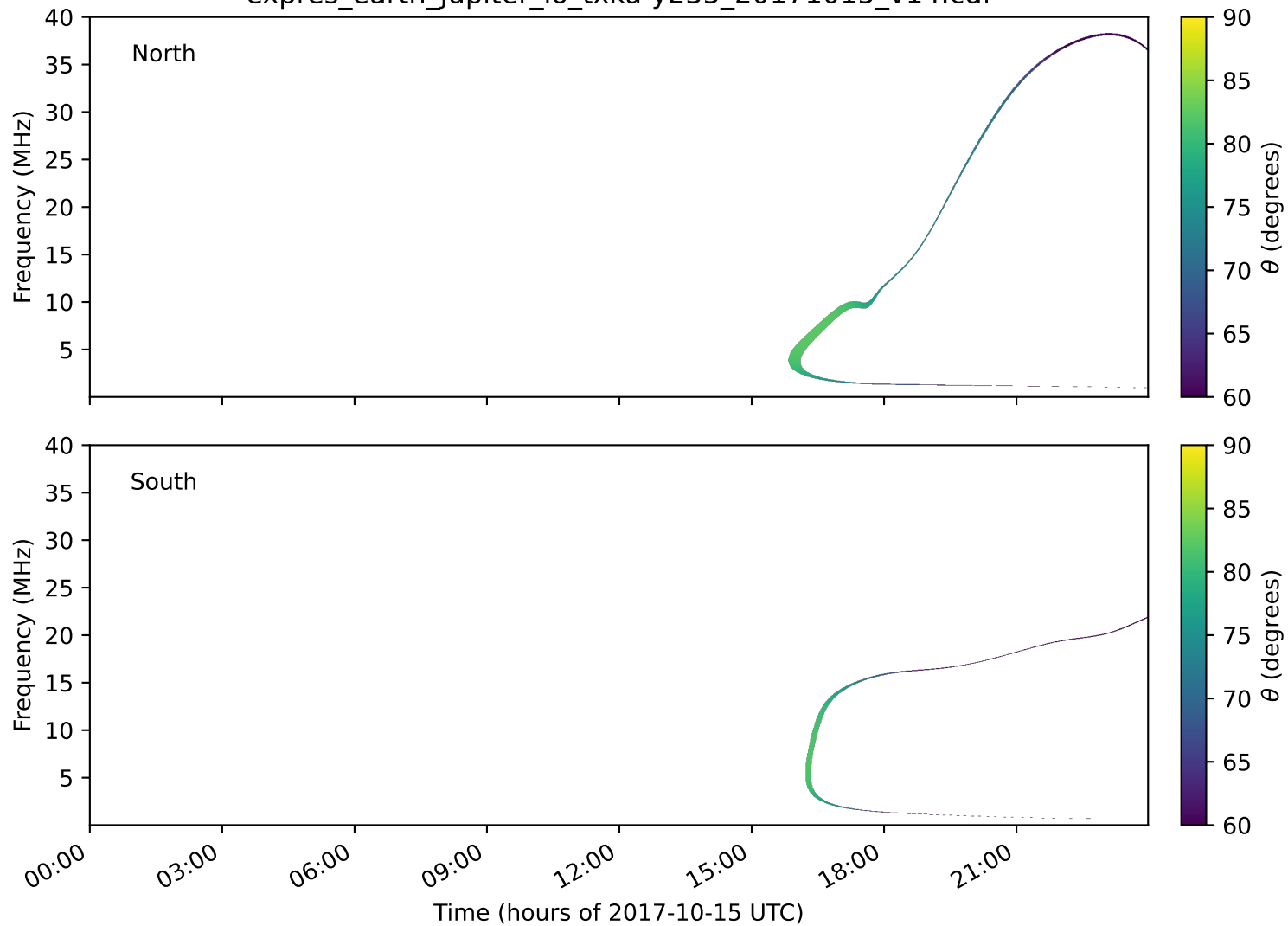
expres_earth_jupiter_io_txka-y235_20171015_v14.cdf
