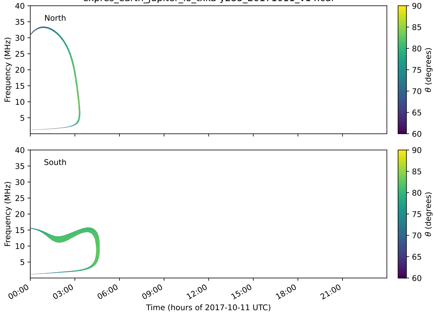
expres_earth_jupiter_io_txka-y235_20171011_v14.cdf
