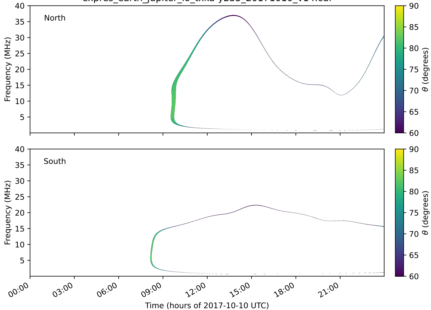
expres_earth_jupiter_io_txka-y235_20171010_v14.cdf
