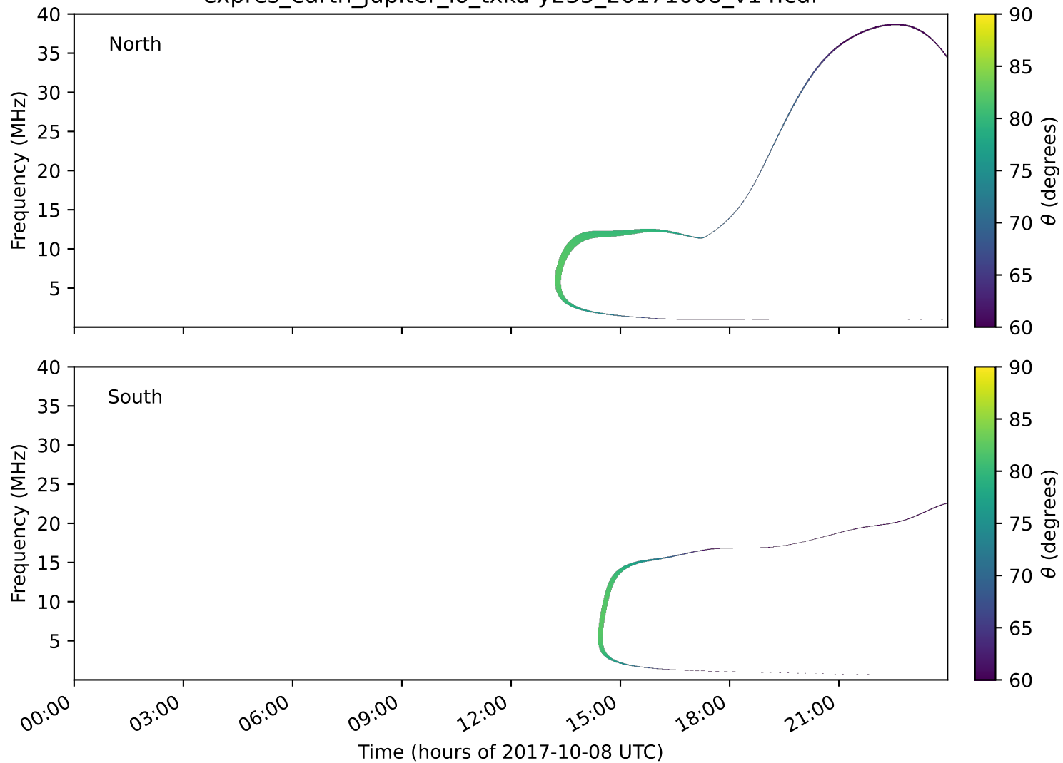
expres_earth_jupiter_io_txka-y235_20171008_v14.cdf
