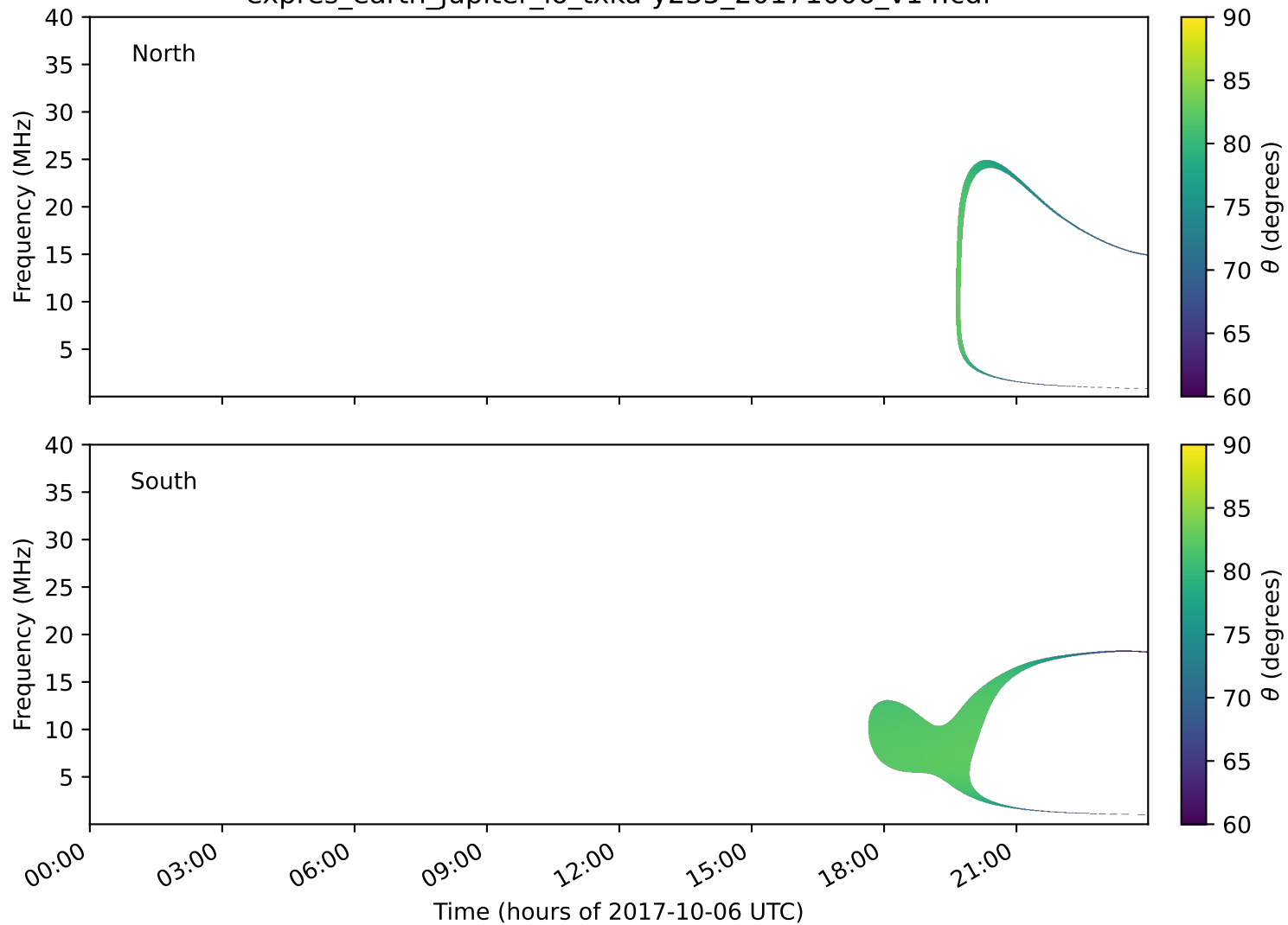
expres_earth_jupiter_io_txka-y235_20171006_v14.cdf
