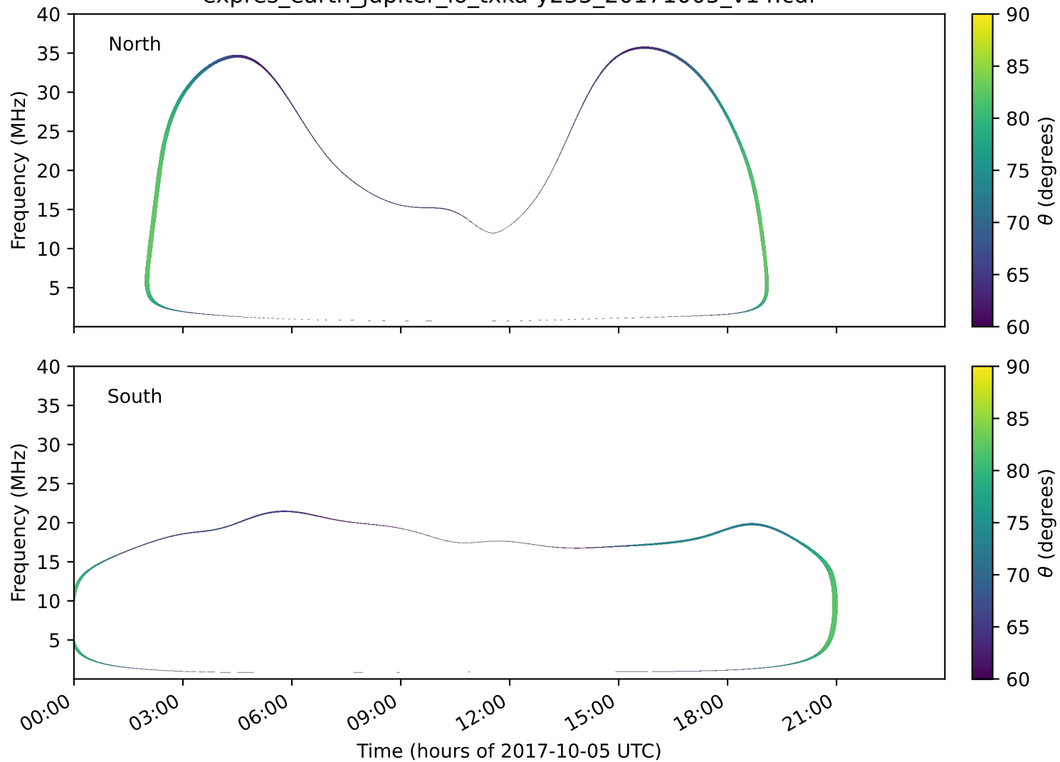
expres_earth_jupiter_io_txka-y235_20171005_v14.cdf
