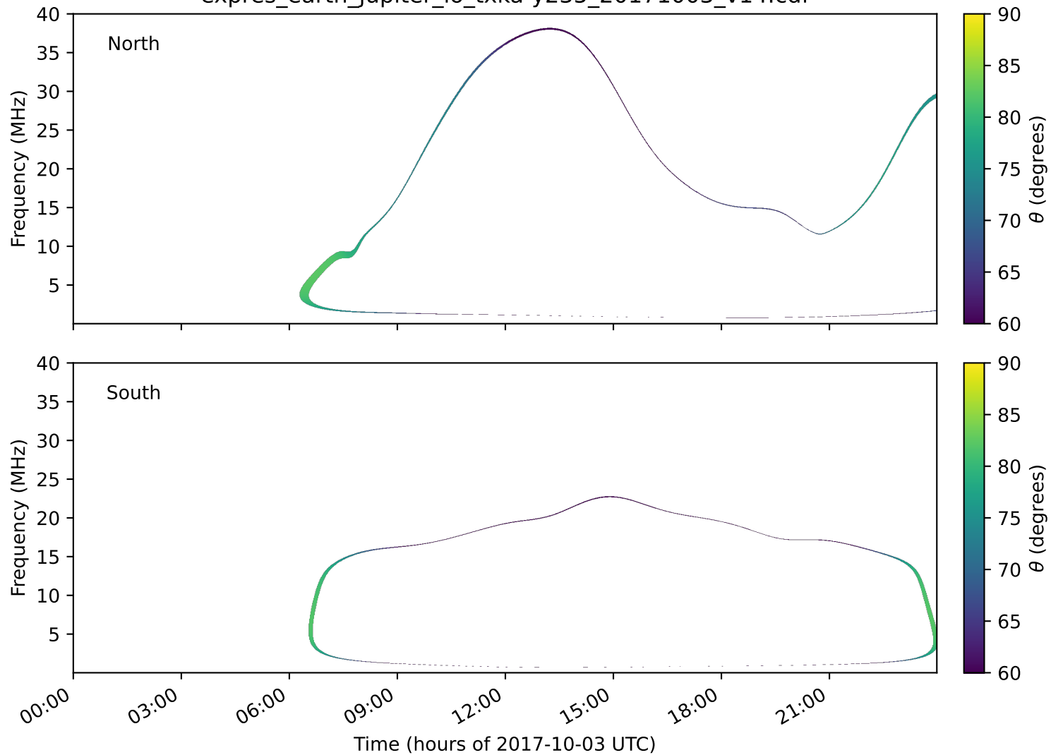
expres_earth_jupiter_io_txka-y235_20171003_v14.cdf
