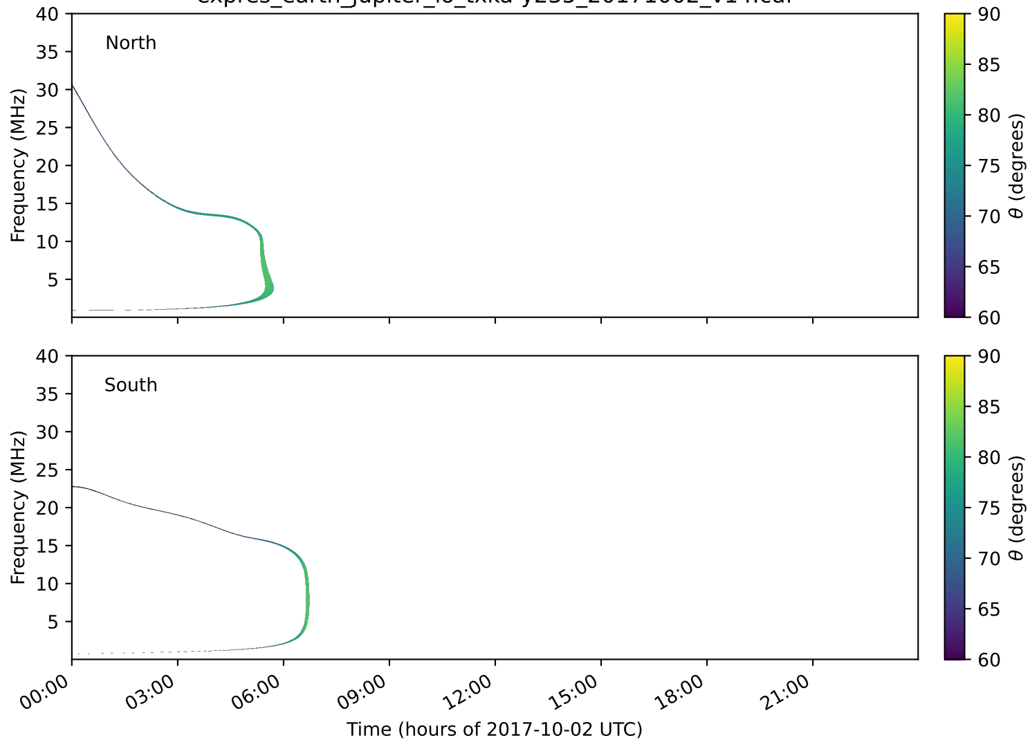
expres_earth_jupiter_io_txka-y235_20171002_v14.cdf
