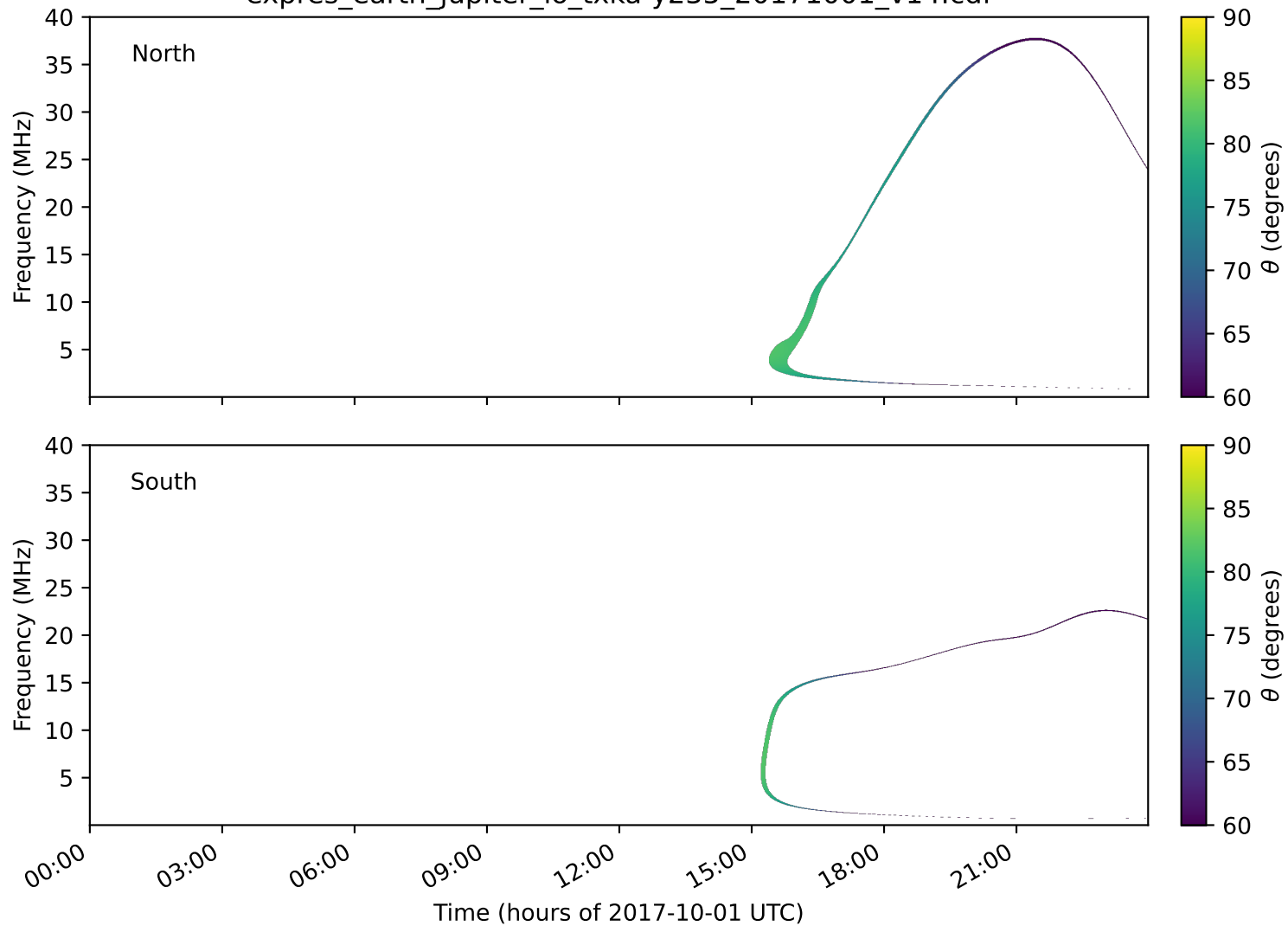
expres_earth_jupiter_io_txka-y235_20171001_v14.cdf
