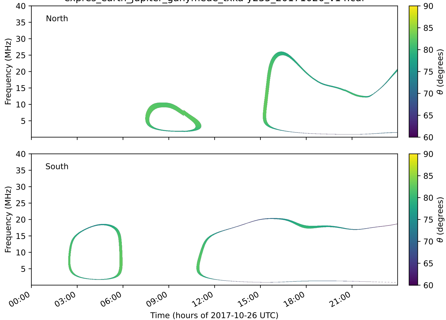
expres_earth_jupiter_ganymede_txka-y235_20171026_v14.cdf
