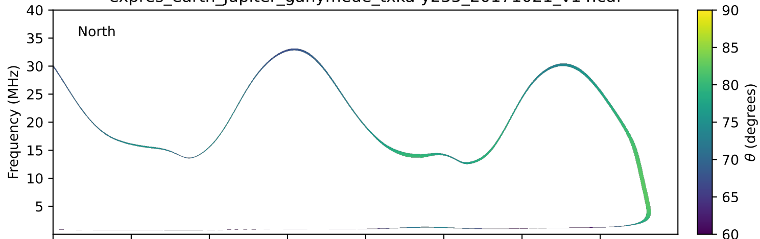
expres_earth_jupiter_ganymede_txka-y235_20171021_v14.cdf
