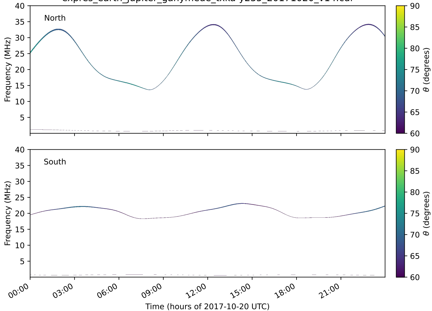
expres_earth_jupiter_ganymede_txka-y235_20171020_v14.cdf
