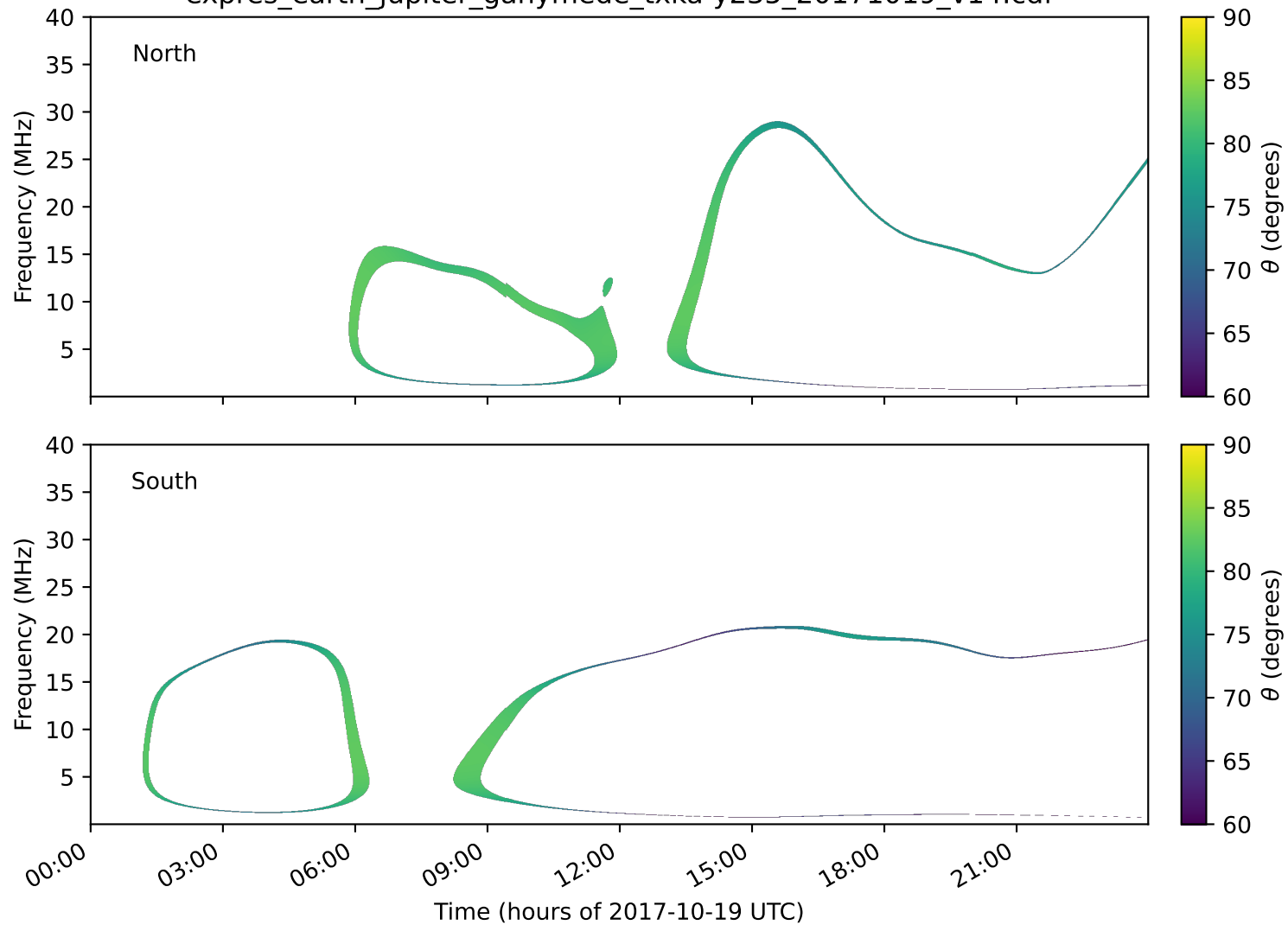
expres_earth_jupiter_ganymede_txka-y235_20171019_v14.cdf
