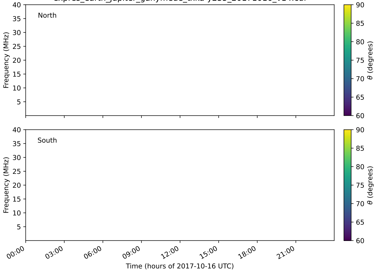
expres_earth_jupiter_ganymede_txka-y235_20171016_v14.cdf
