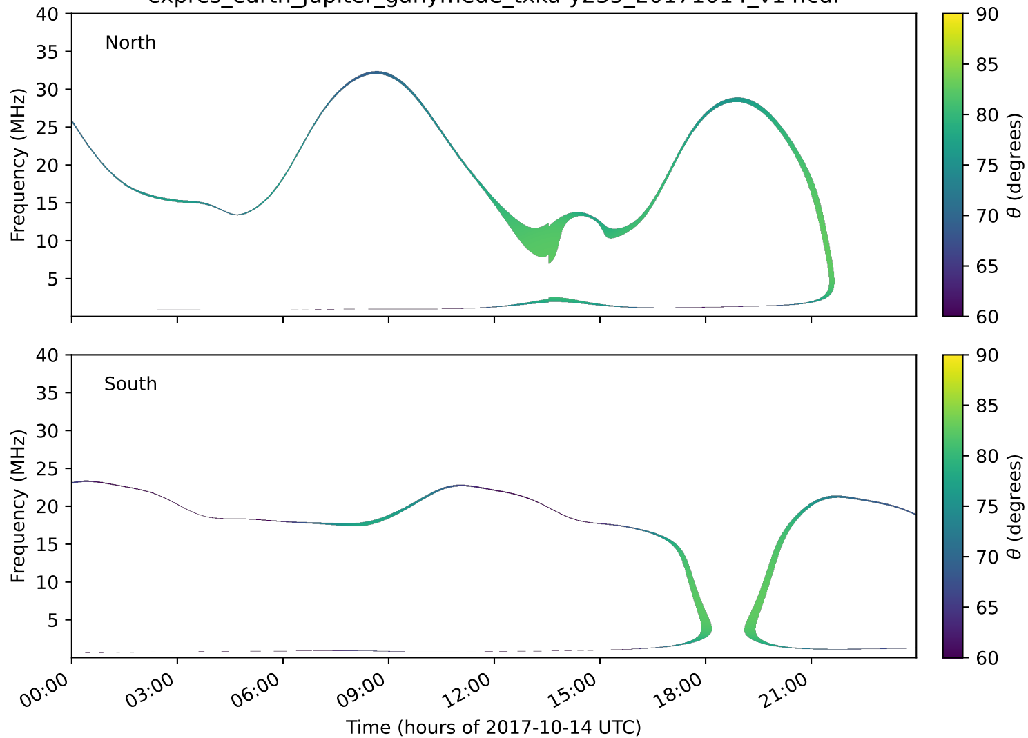
expres_earth_jupiter_ganymede_txka-y235_20171014_v14.cdf
