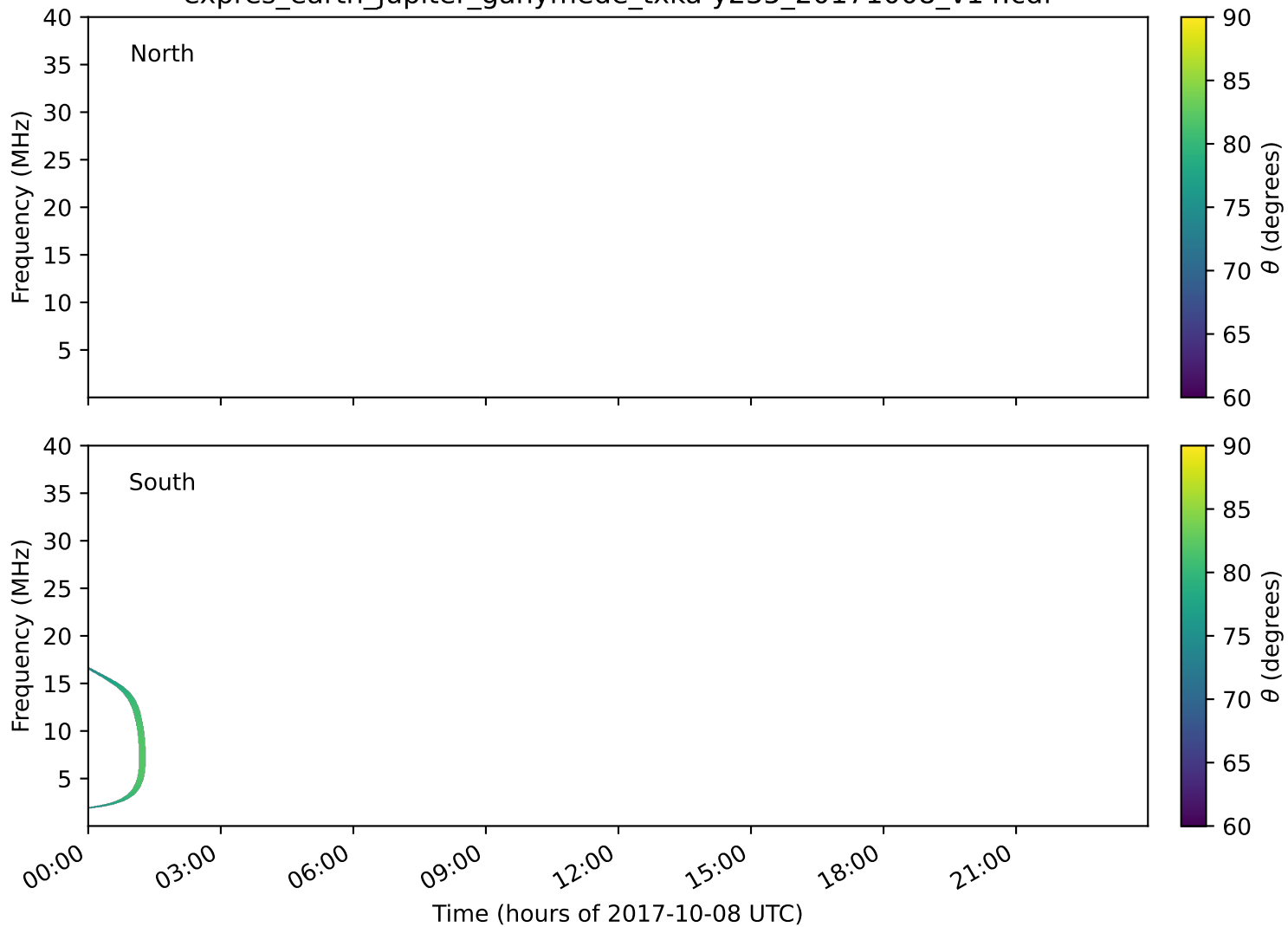
expres_earth_jupiter_ganymede_txka-y235_20171008_v14.cdf
