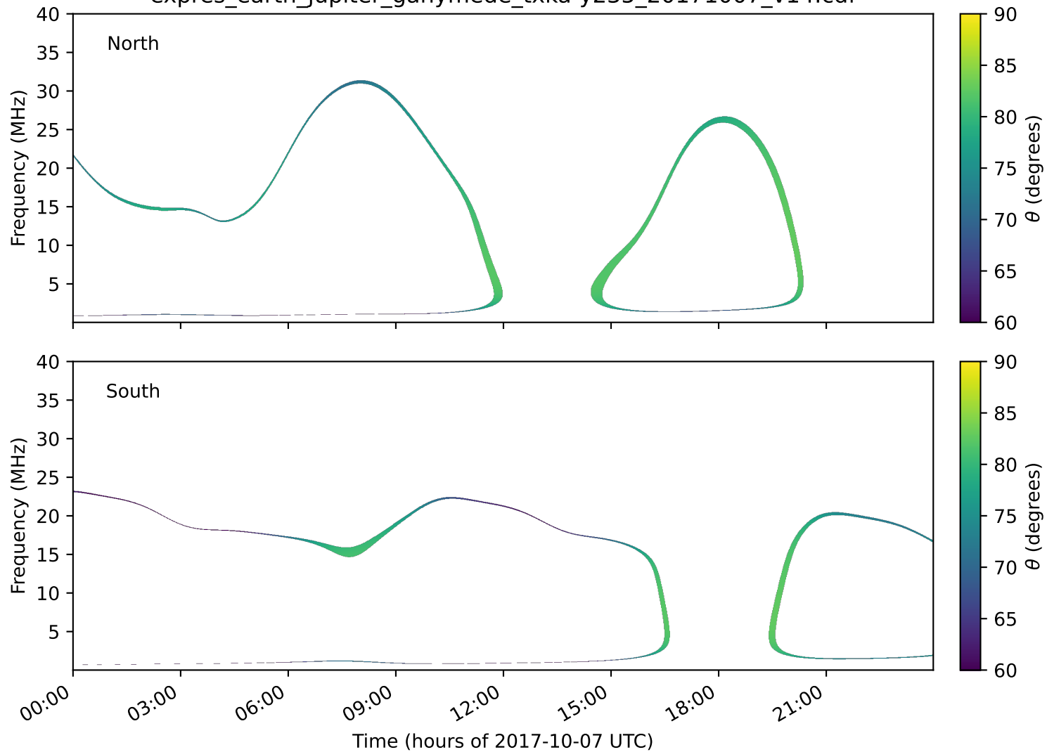
expres_earth_jupiter_ganymede_txka-y235_20171007_v14.cdf
