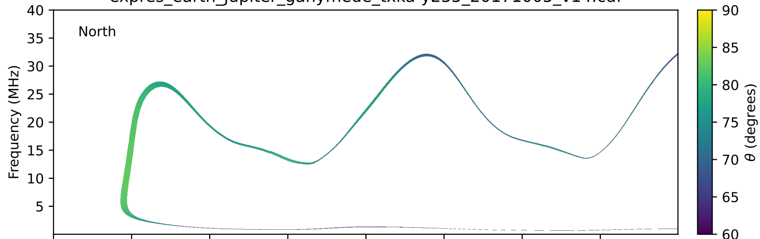
expres_earth_jupiter_ganymede_txka-y235_20171005_v14.cdf
