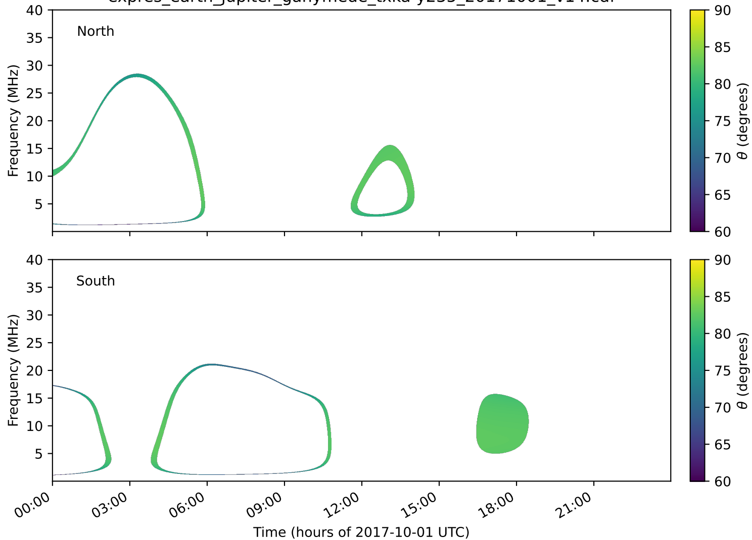
expres_earth_jupiter_ganymede_txka-y235_20171001_v14.cdf
