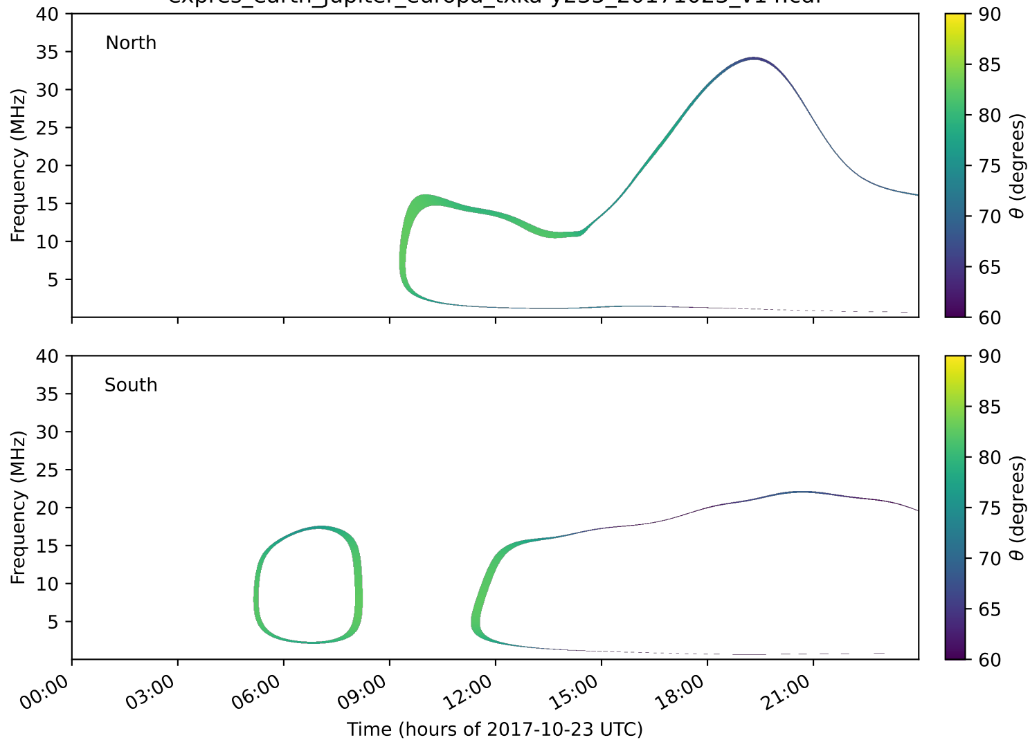
expres_earth_jupiter_europa_txka-y235_20171023_v14.cdf
