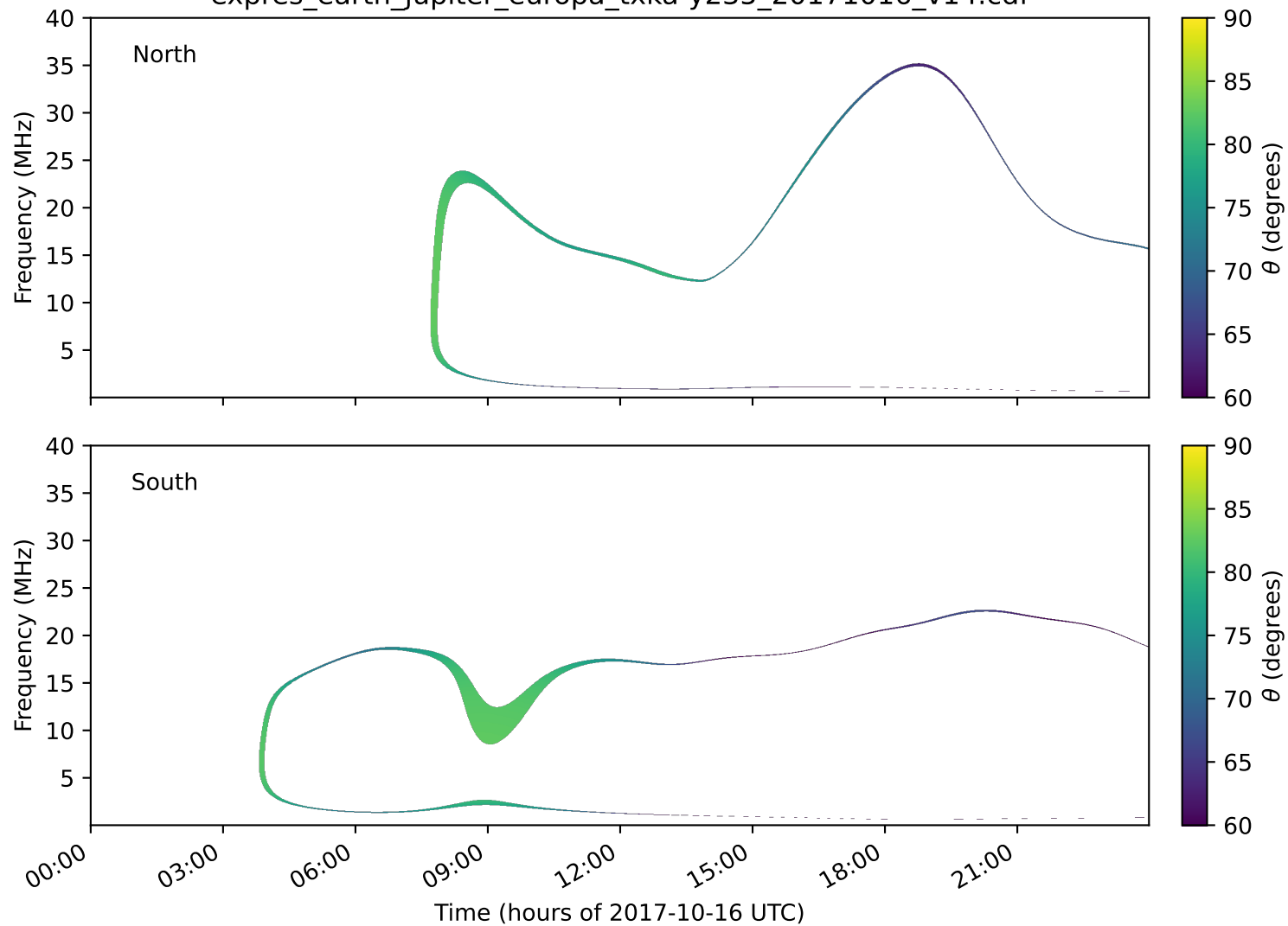
expres_earth_jupiter_europa_txka-y235_20171016_v14.cdf
