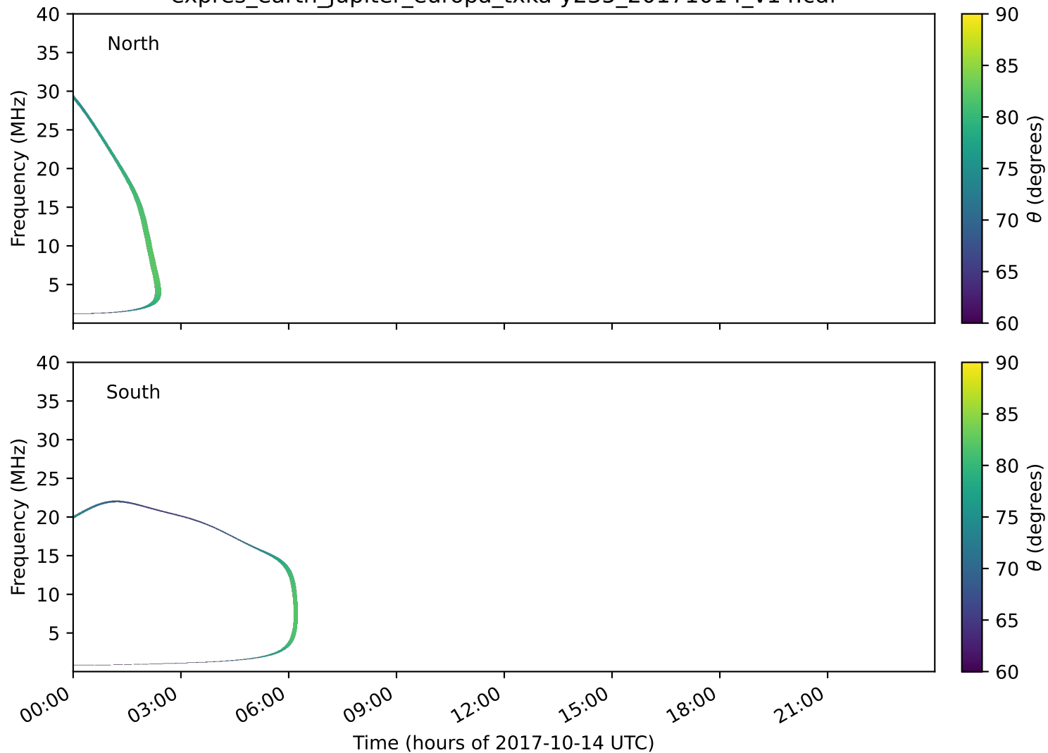
expres_earth_jupiter_europa_txka-y235_20171014_v14.cdf
