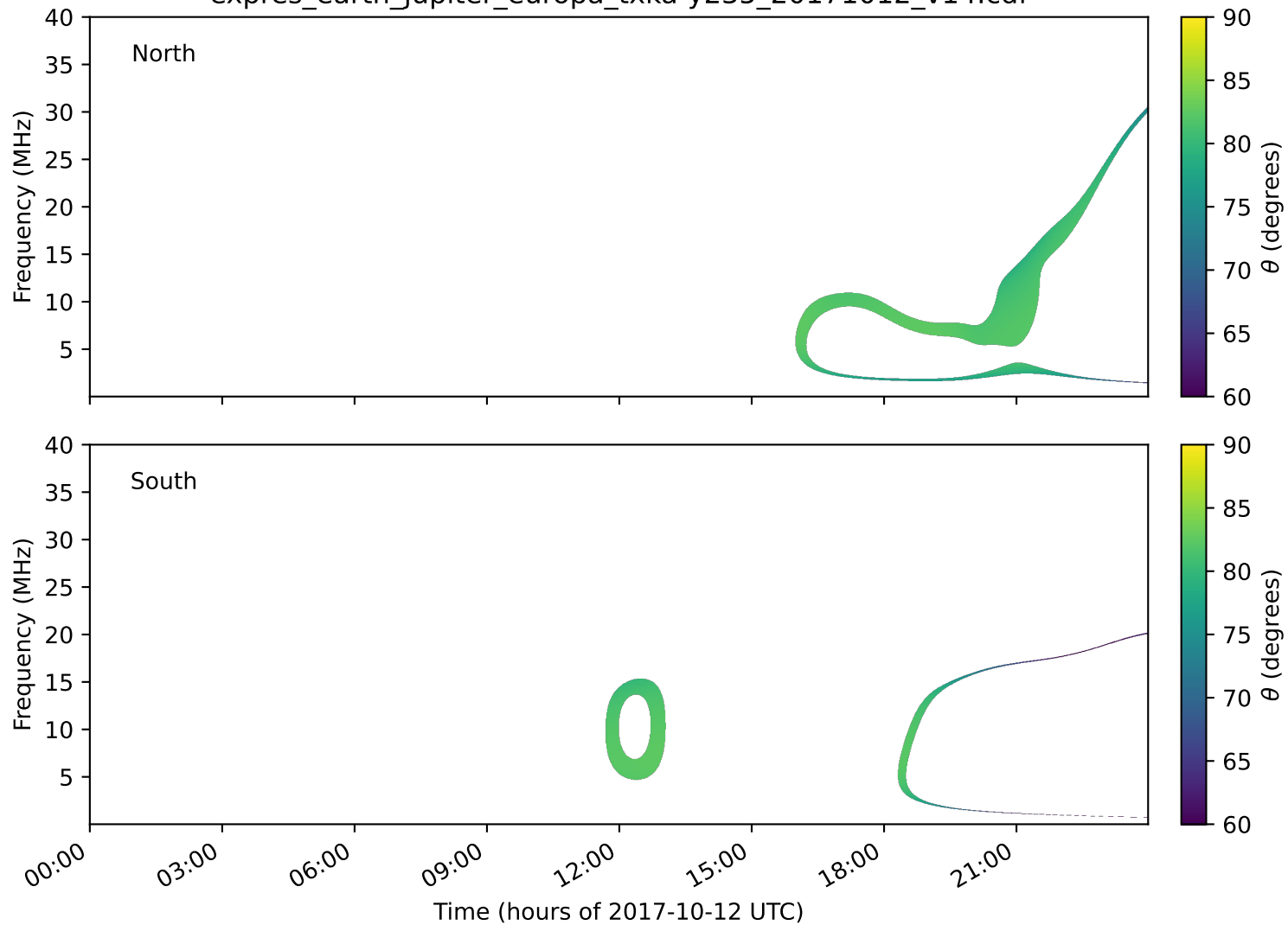
expres_earth_jupiter_europa_txka-y235_20171012_v14.cdf
