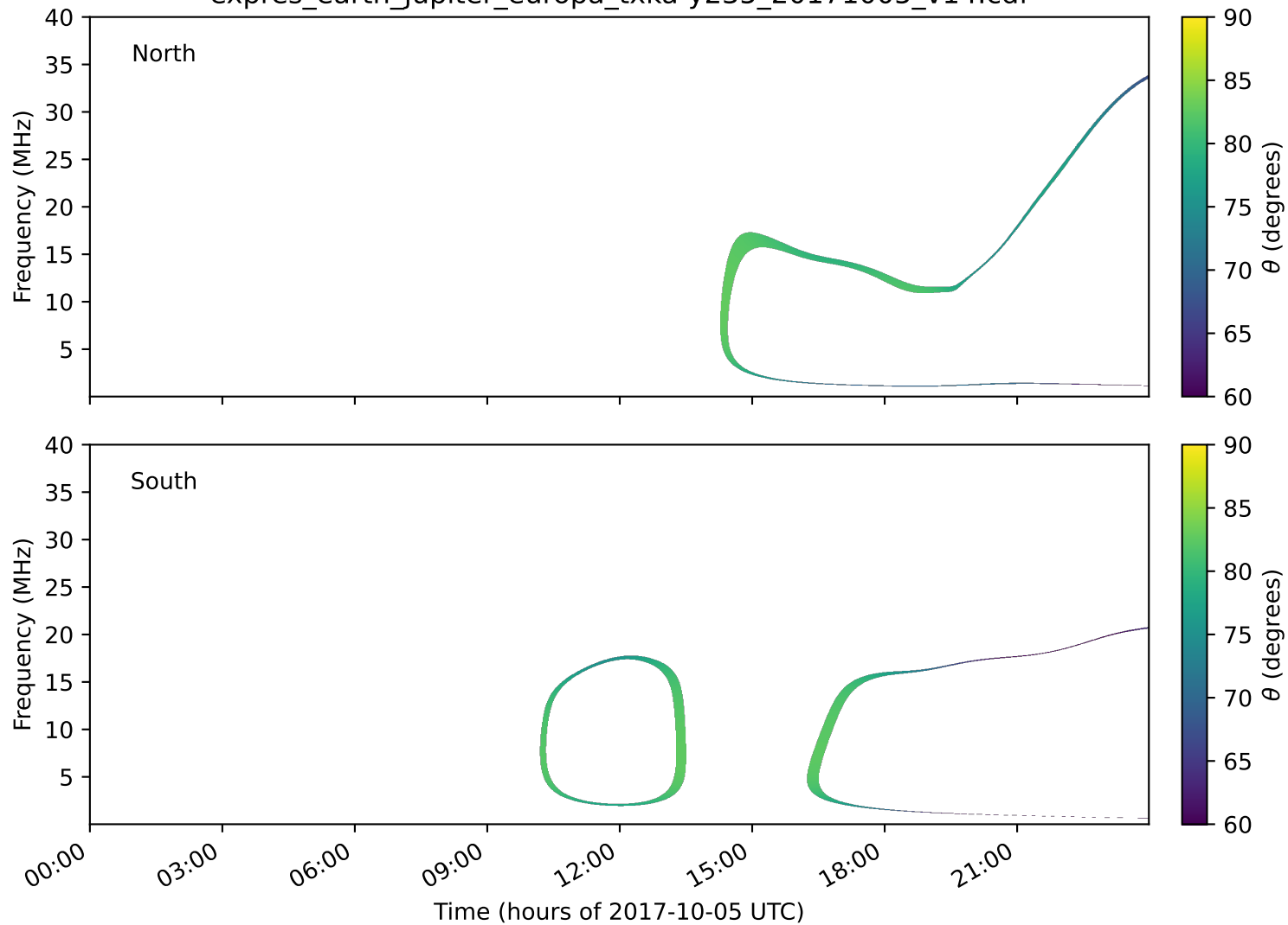
expres_earth_jupiter_europa_txka-y235_20171005_v14.cdf
