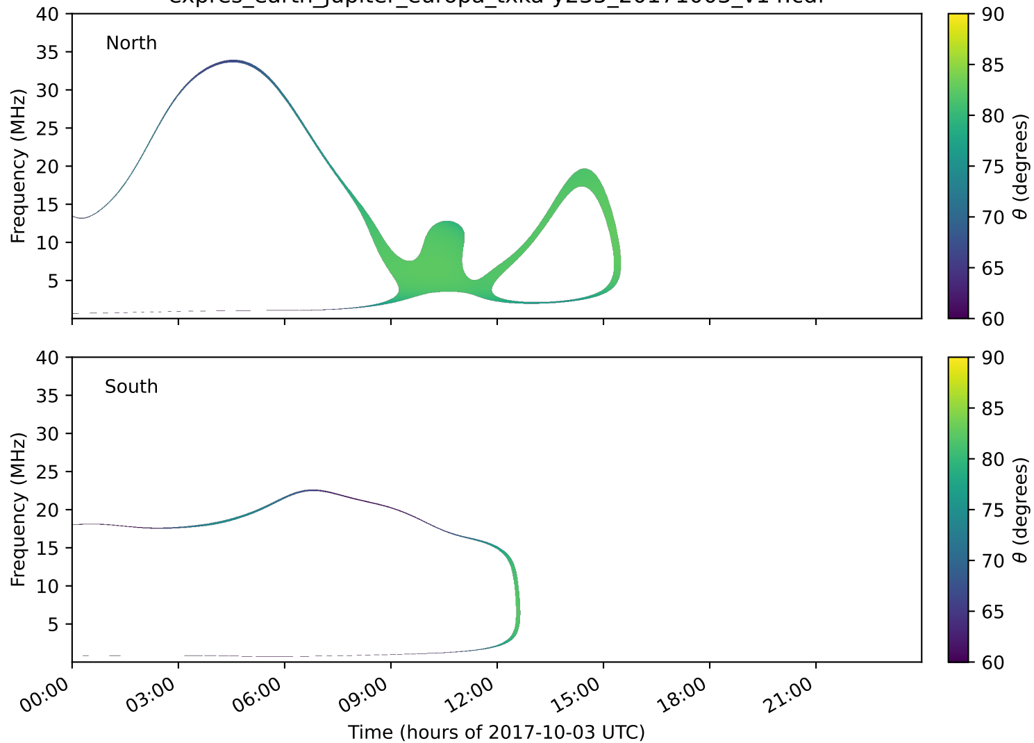
expres_earth_jupiter_europa_txka-y235_20171003_v14.cdf
