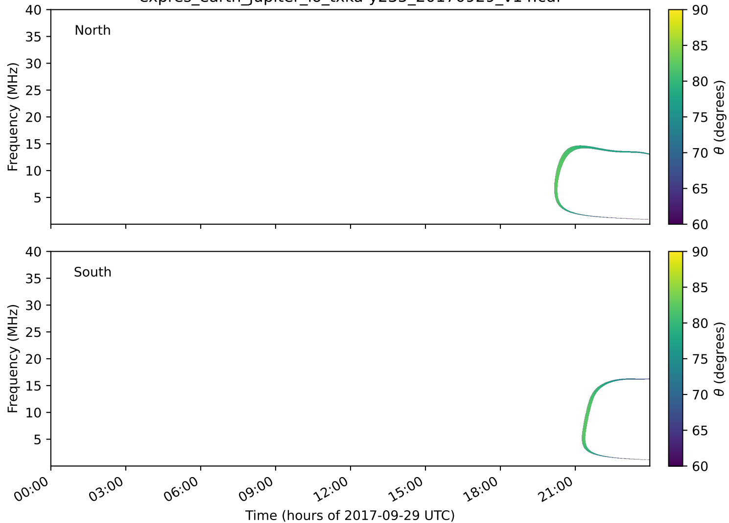
expres_earth_jupiter_io_txka-y235_20170929_v14.cdf
