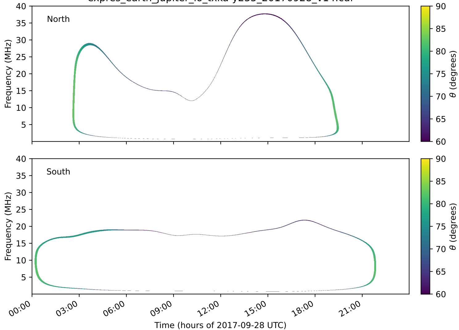
expres_earth_jupiter_io_txka-y235_20170928_v14.cdf
