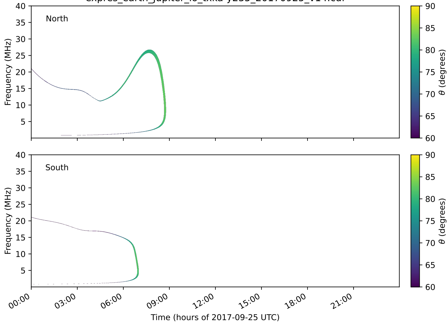
expres_earth_jupiter_io_txka-y235_20170925_v14.cdf
