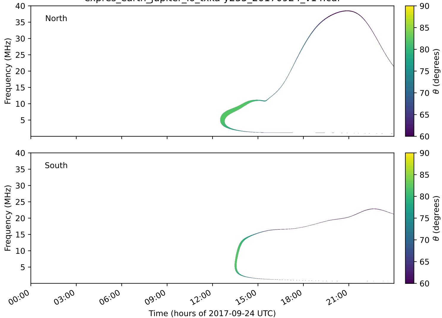
expres_earth_jupiter_io_txka-y235_20170924_v14.cdf
