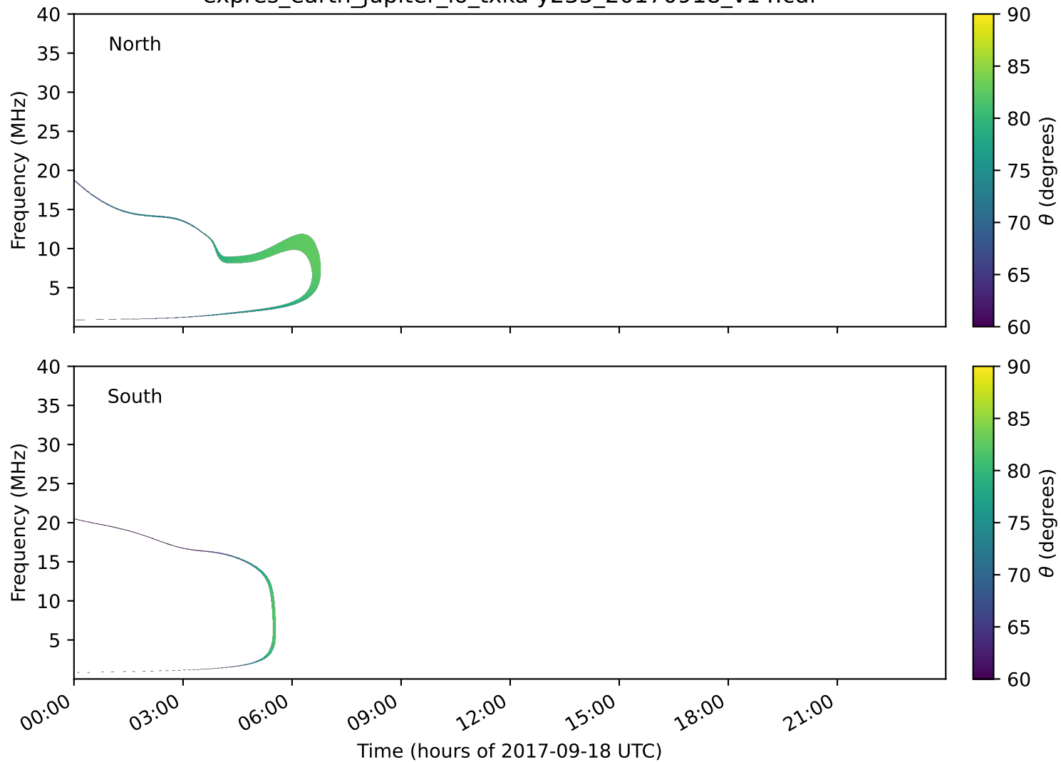
expres_earth_jupiter_io_txka-y235_20170918_v14.cdf
