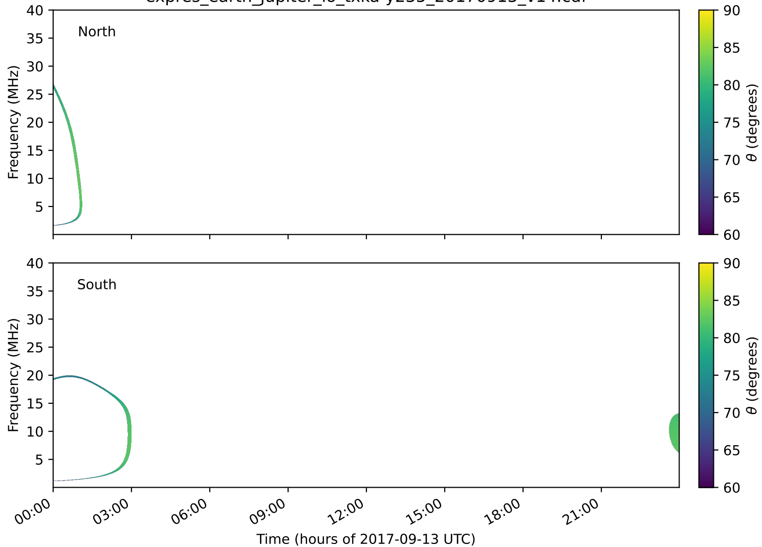
expres_earth_jupiter_io_txka-y235_20170913_v14.cdf
