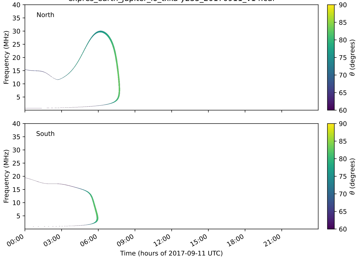
expres_earth_jupiter_io_txka-y235_20170911_v14.cdf
